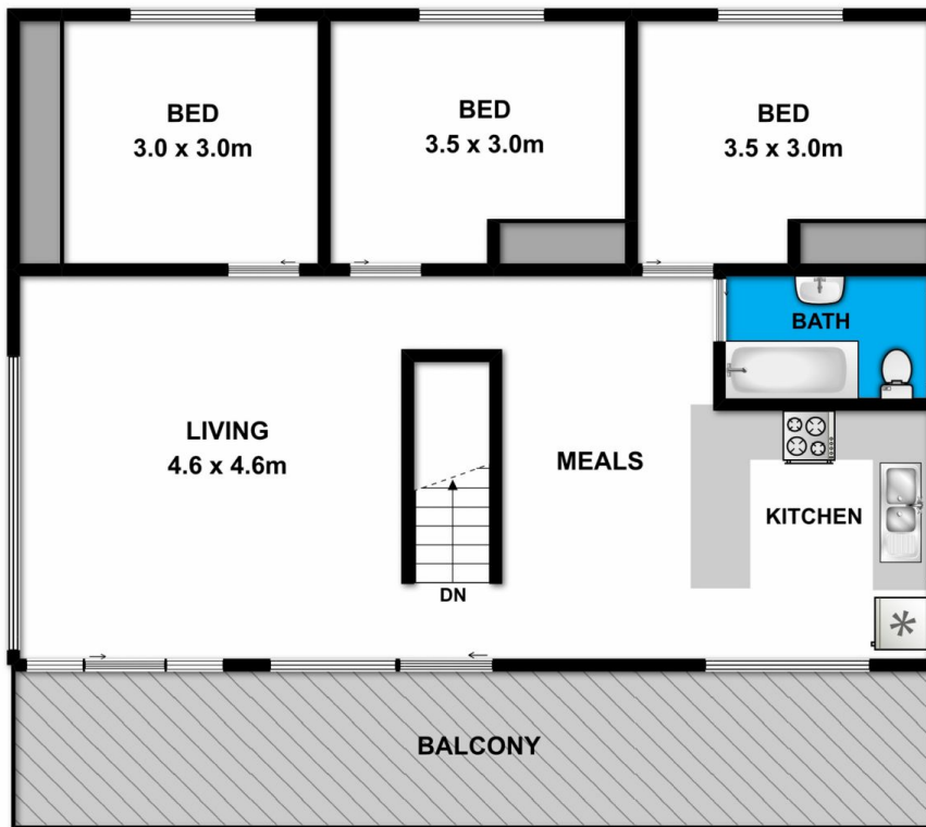
First Floor
